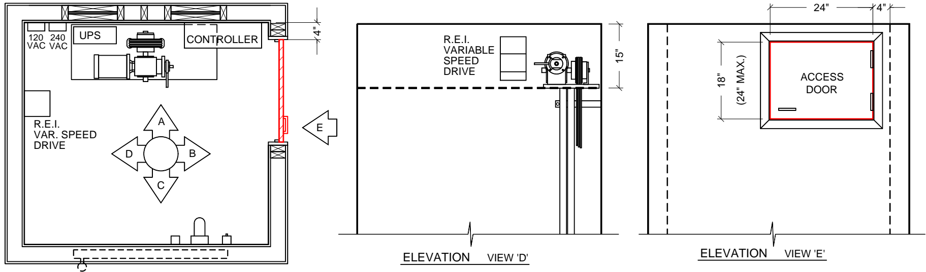
PLAN VIEW
